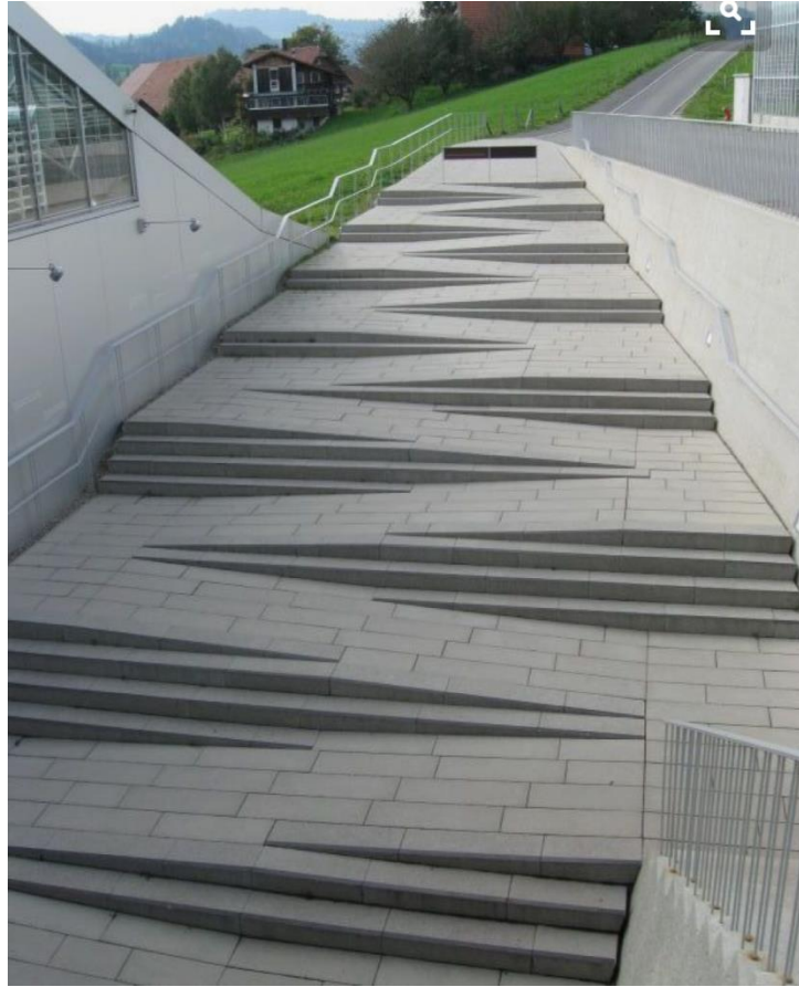
RAMP STAIR
